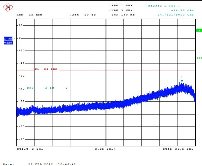
Band7-10MHz-16QAM-21100-1RB#0-Range1:3000~26500MHz
