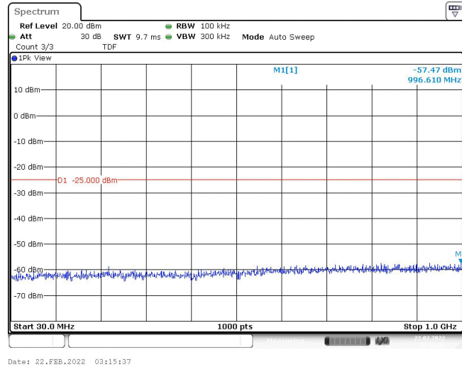
Band7-10MHz-QPSK-21100-1RB#0-Range1:30~1000MHz
