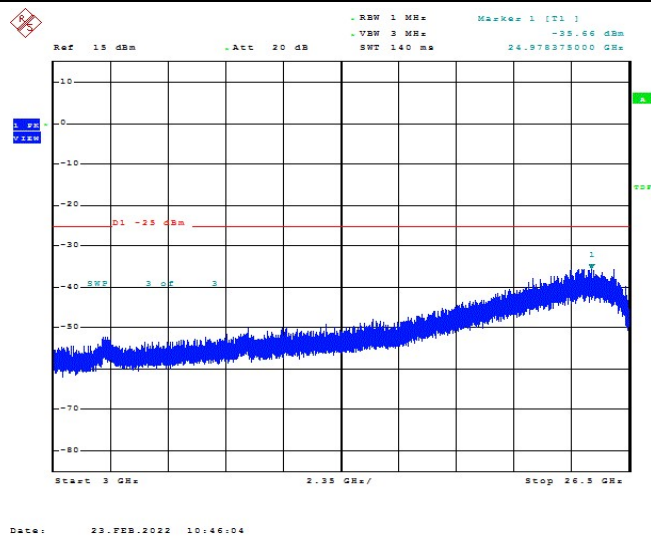
Band7-10MHz-16QAM-20800-1RB#0-Range1:3000~26500MHz
