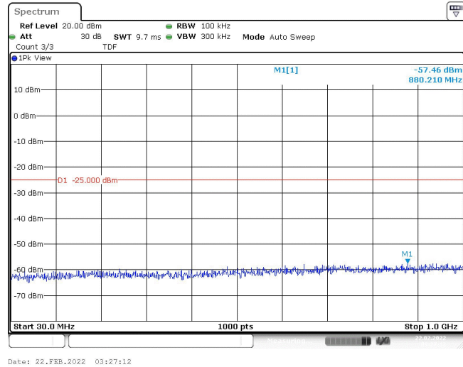
Band7-15MHz-QPSK-21100-1RB#0-Range1:30~1000MHz
