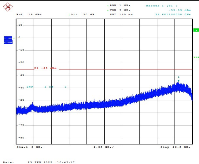
Band7-10MHz-16QAM-21400-1RB#0-Range1:3000~26500MHz
