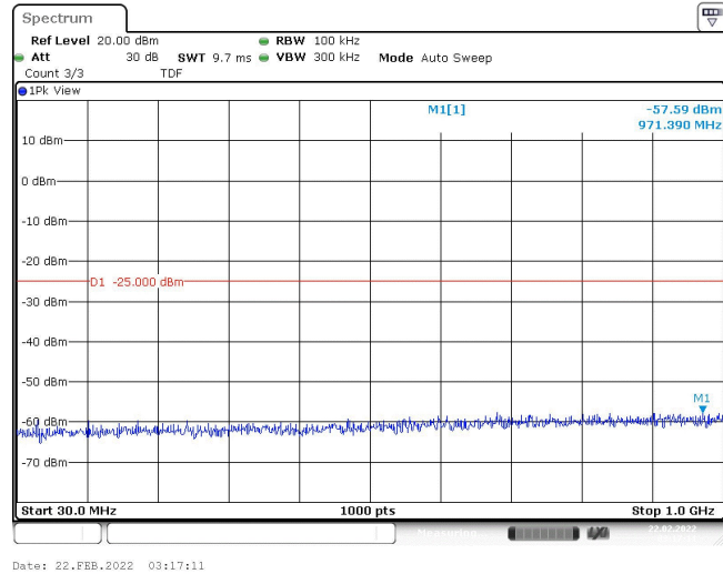
Band7-10MHz-16QAM-21400-1RB#0-Range1:30~1000MHz
