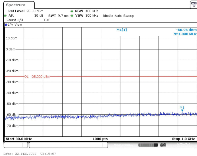
Band7-10MHz-16QAM-21100-1RB#0-Range1:30~1000MHz
