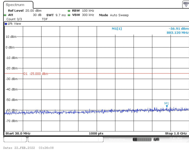
Band7-15MHz-QPSK-20825-1RB#0-Range1:30~1000MHz
