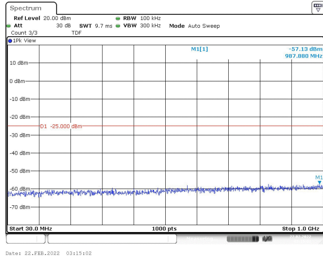
Band7-10MHz-16QAM-20800-1RB#0-Range1:30~1000MHz
