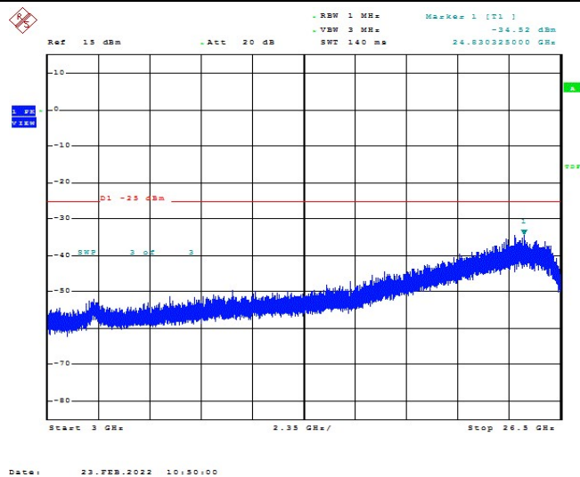
Band7-15MHz-QPSK-21100-1RB#0-Range1:3000~26500MHz
