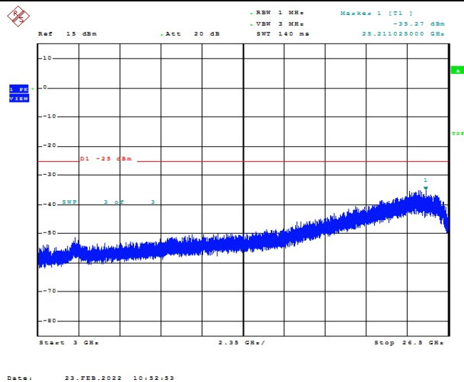
Band7-20MHz-16QAM-20850-1RB#0-Range1:3000~26500MHz
