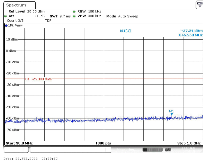
Band7-20MHz-QPSK-21350-1RB#0-Range1:30~1000MHz
