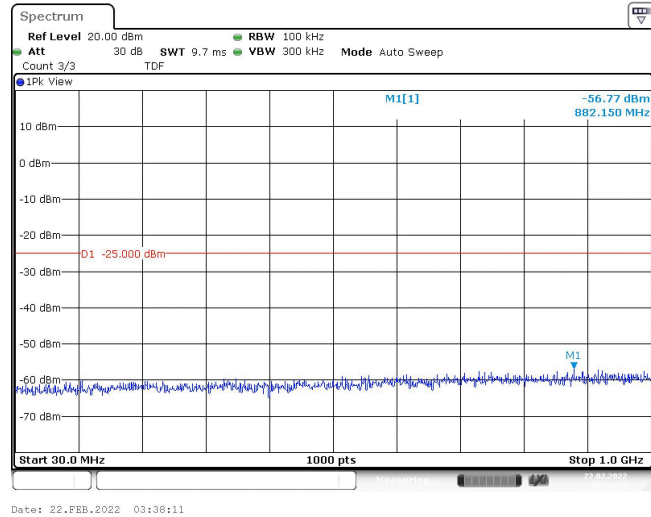
Band7-20MHz-16QAM-20850-1RB#0-Range1:30~1000MHz
