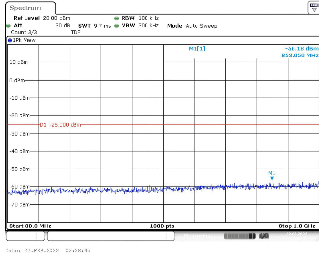
Band7-15MHz-16QAM-21375-1RB#0-Range1:30~1000MHz
