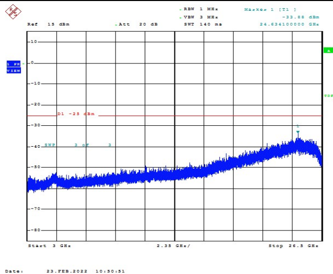
Band7-15MHz-16QAM-21375-1RB#0-Range1:3000~26500MHz
