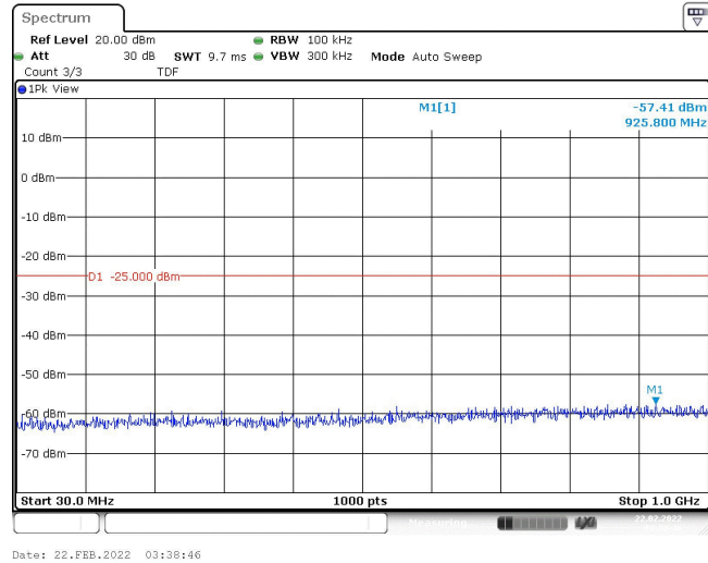
Band7-20MHz-QPSK-21100-1RB#0-Range1:30~1000MHz
