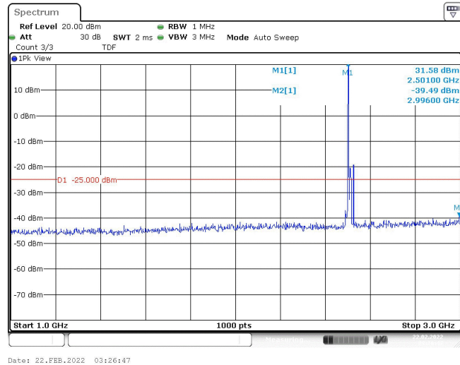
Band7-15MHz-16QAM-20825-1RB#0-Range2:1000~3000MHz
