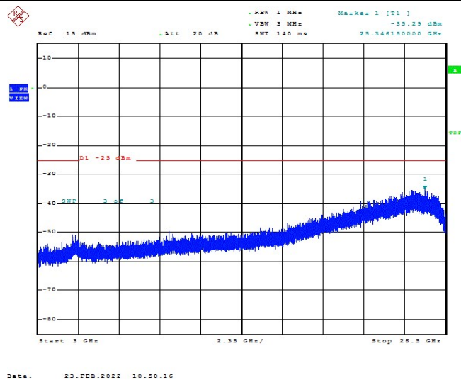
Band7-15MHz-16QAM-21100-1RB#0-Range1:3000~26500MHz
