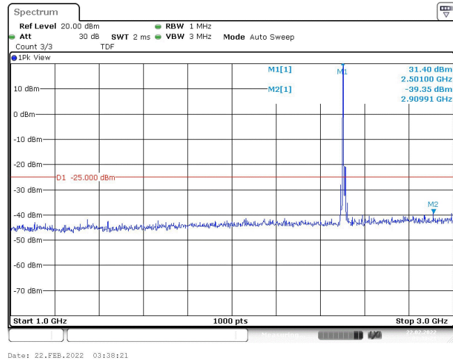
Band7-20MHz-16QAM-20850-1RB#0-Range2:1000~3000MHz
