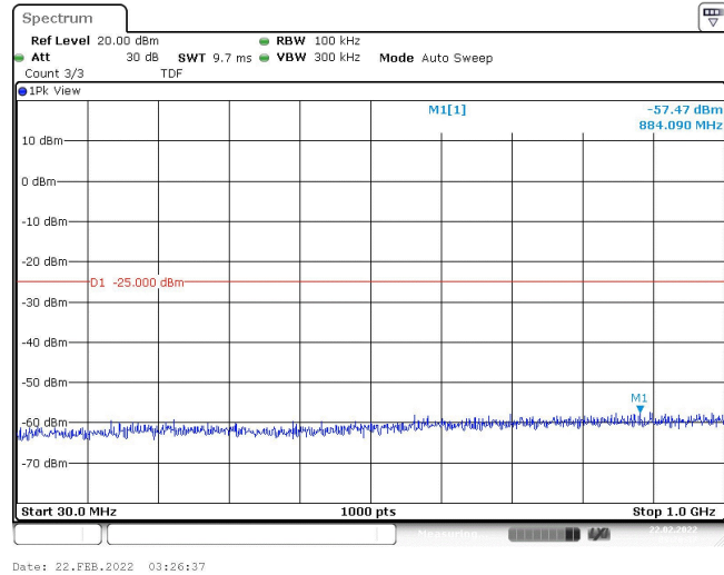
Band7-15MHz-16QAM-20825-1RB#0-Range1:30~1000MHz
