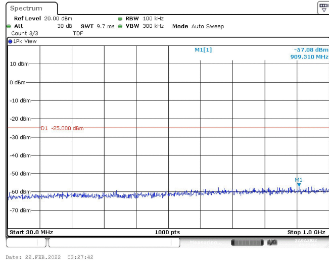
Band7-15MHz-16QAM-21100-1RB#0-Range1:30~1000MHz
