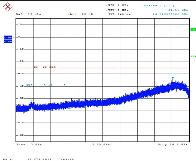
Band7-15MHz-16QAM-20825-1RB#0-Range1:3000~26500MHz
