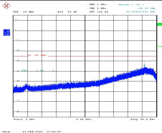
Band7-20MHz-16QAM-21350-1RB#0-Range1:3000~26500MHz
