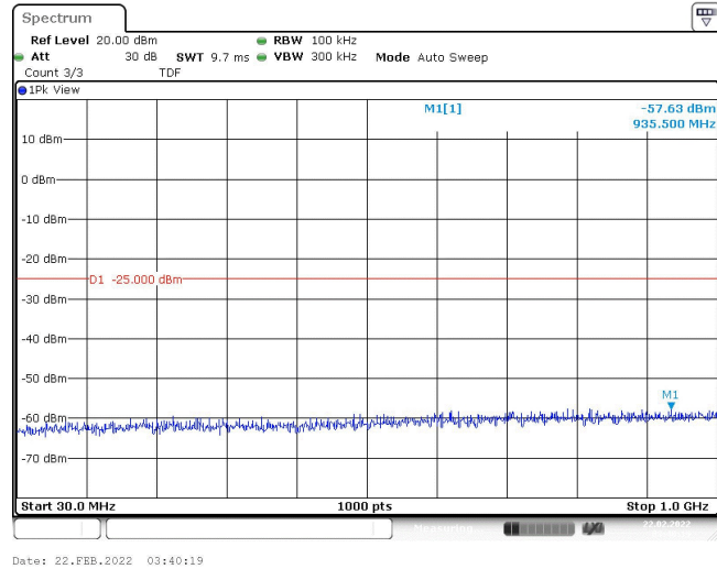
Band7-20MHz-16QAM-21350-1RB#0-Range1:30~1000MHz
