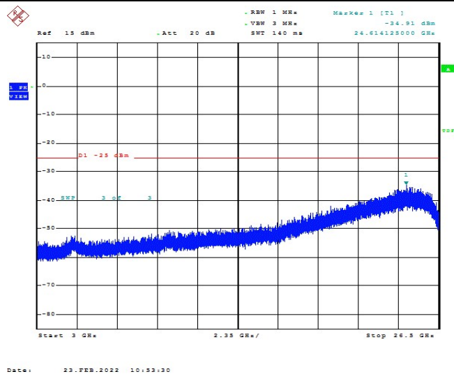
Band7-20MHz-16QAM-21100-1RB#0-Range1:3000~26500MHz
