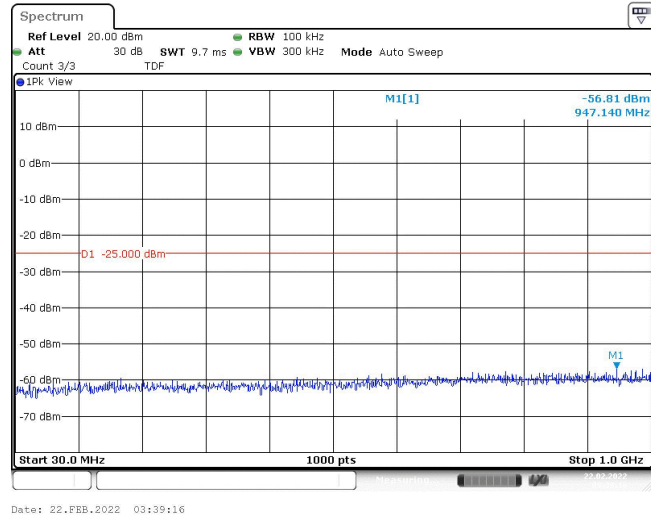
Band7-20MHz-16QAM-21100-1RB#0-Range1:30~1000MHz
