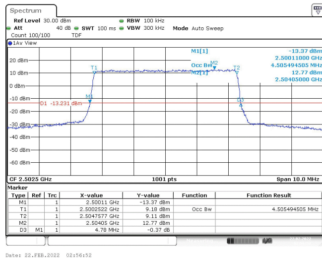
Band7-5MHz-QPSK-20775-25RB#0-4.505
