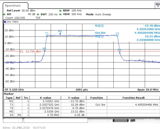
Band7-5MHz-QPSK-21100-25RB#0-4.496
