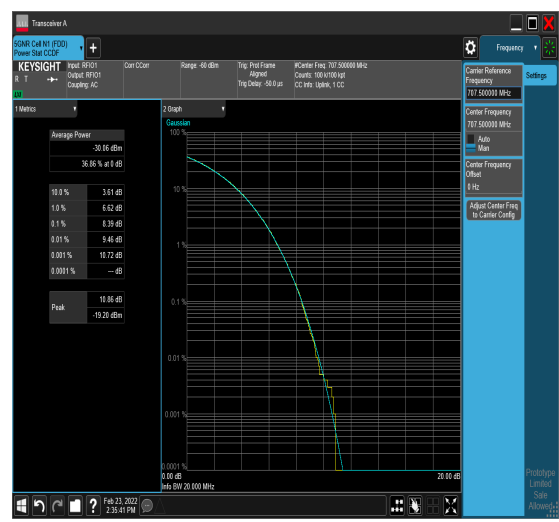
1-N12-PC3-15-15-M-9-CP-256QAM-Outer_Full-79@0-8.39-100%-0.00-8.39-PASS≤13
