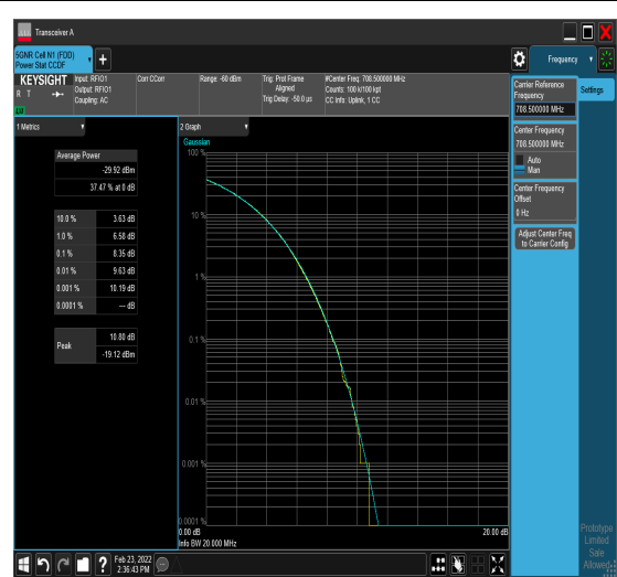
1-N12-PC3-15-15-H-2-DFT-QPSK-Outer_Full
