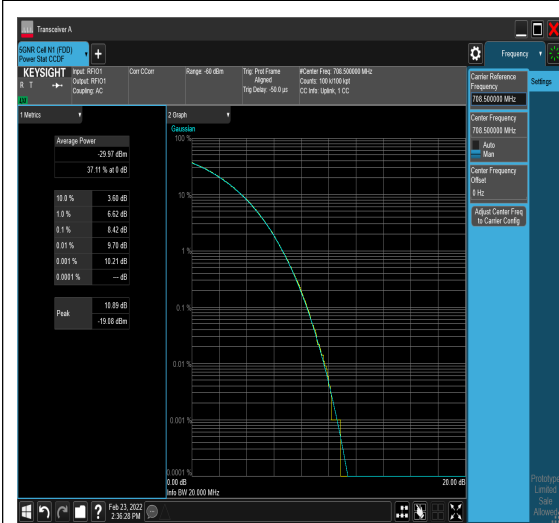
1-N12-PC3-15-15-H-1-DFT-PI2BPSK-Outer_
