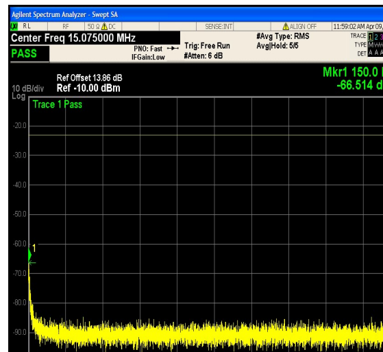
1-N12-PC3-15-5-M-22-CP-64QAM-Edge_1R B_Left-1@0-0.15-30-Ant1--66.51--23-PASS
