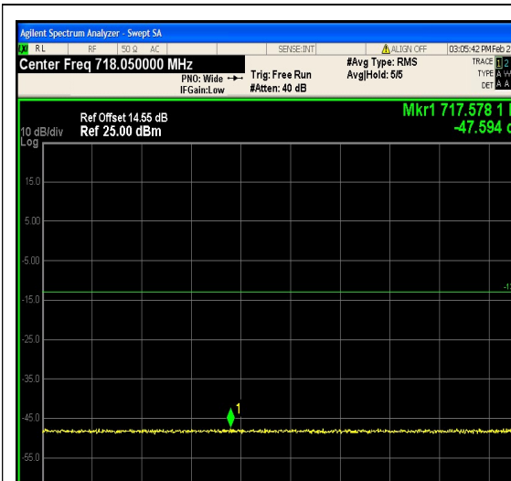
1-N12-PC3-15-10-H-2-DFT-PI2BPSK-Edge_1RB_Right-1@51-Ant1-716.1~720(717.5781 MHz,-47.59MHz,Limit-13,Margin[34.59])-PAS S-see graph
