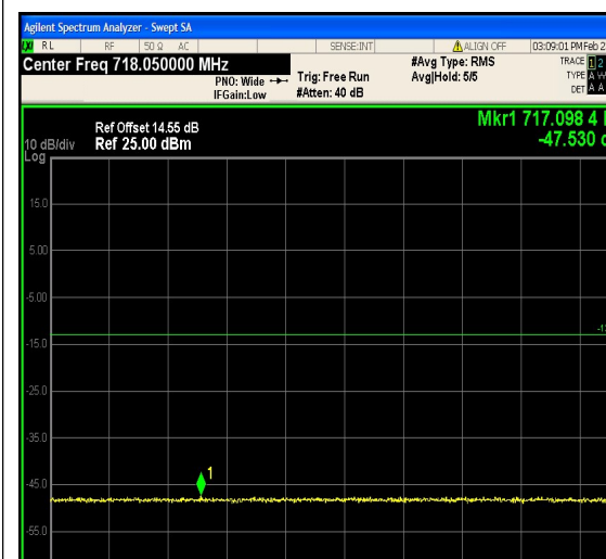
1-N12-PC3-15-10-H-5-CP-QPSK-Edge_1RB_Right-1@51-Ant1-716.1~720(717.0984MHz,-47.53MHz,Limit-13,Margin[34.53])-PASS-se e graph
