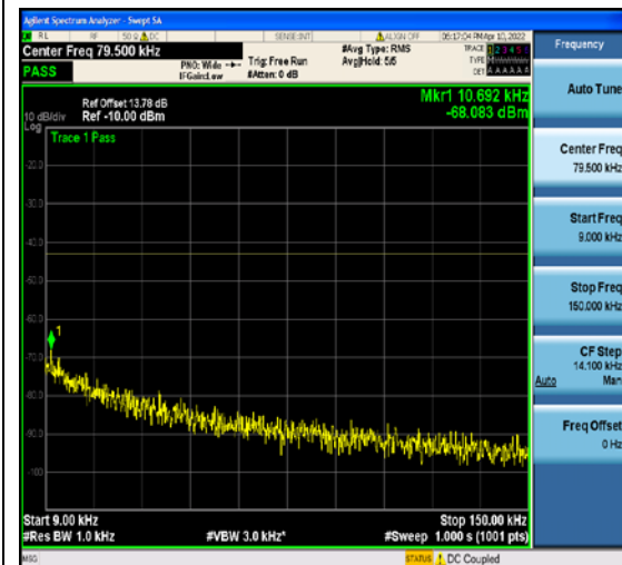
1-N2-PC3-15-20-L-4-DFT-QPSK-Edge_1RB_ Left-1@0-0.009-0.15-Ant1--68.08--43-PASS
