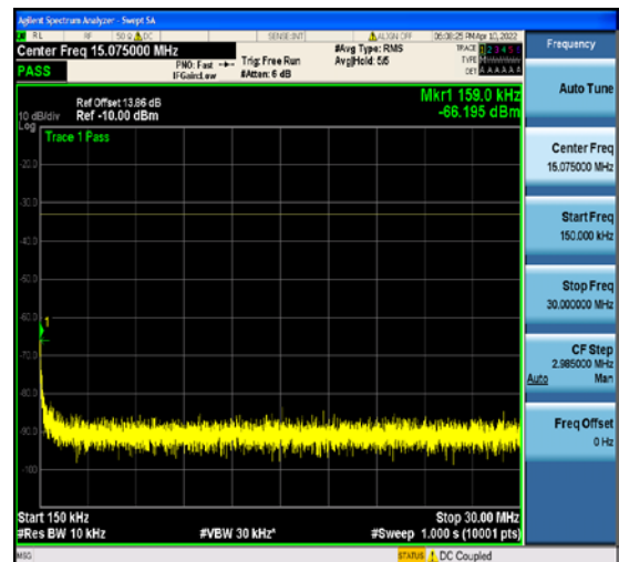
1-N2-PC3-15-15-M-4-DFT-QPSK-Edge_1RB _Left-1@0-0.15-30-Ant1--66.19--33-PASS
