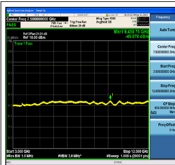
1-N2-PC3-15-15-H-5-DFT-QPSK-Edge_1RB _Right-1@78-3000-12000-Ant1--45.08--13-P ASS
