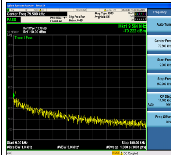
1-N2-PC3-15-15-M-4-DFT-QPSK-Edge_1RB _Left-1@0-0.009-0.15-Ant1--70.22--43-PASS
