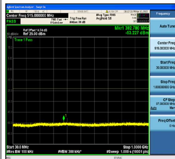
1-N2-PC3-15-20-L-4-DFT-QPSK-Edge_1RB_ Left-1@0-0.009-0.15-Ant1--68.08--43-PASS
