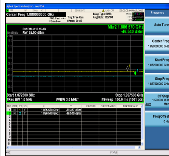
1-N2-PC3-15-5-M-8-CP-64QAM-Out_2 5@0-Ant1-8.20-1%-20.00--11.80-PASS-≤13
