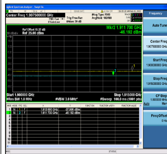
1-N2-PC3-15-5-H-1-DFT-PI2BPSK-Out_Fu
