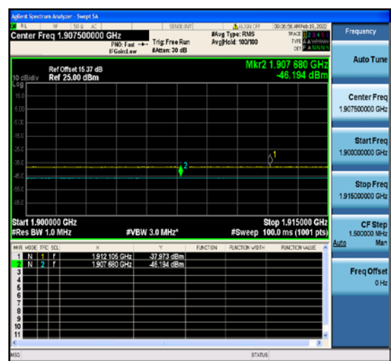
1-N2-PC3-15-5-H-2-DFT-QPSK-Out_Full-2
