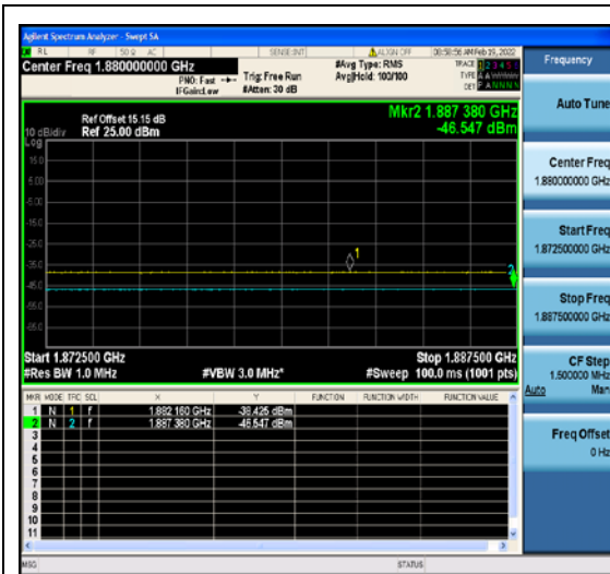
1-N2-PC3-15-5-M-6-CP-QPSK-Out_25 @0-Ant1-8.12-1%-20.00--11.88-PASS-≤13
