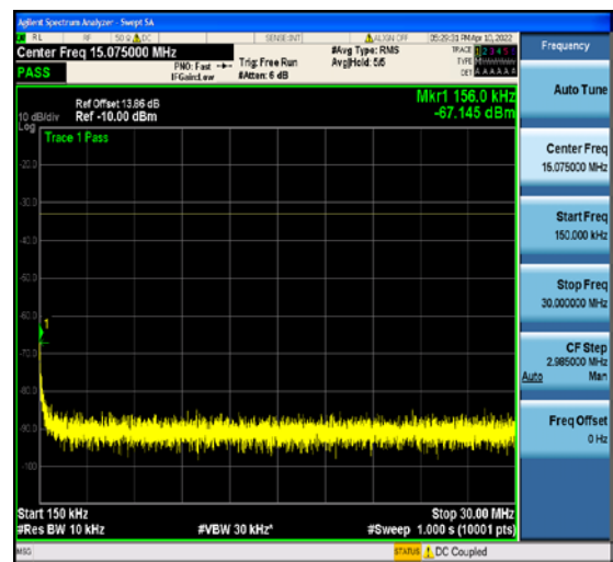
1-N2-PC3-15-5-L-5-DFT-QPSK-Edge_1RB_ Right-1@24-0.15-30-Ant1--67.14--33-PASS
