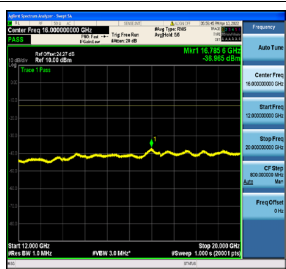
1-N2-PC3-15-10-M-5-DFT-QPSK-Edge_1RB _Right-1@51-12000-20000-Ant1--36.97--13- PASS
