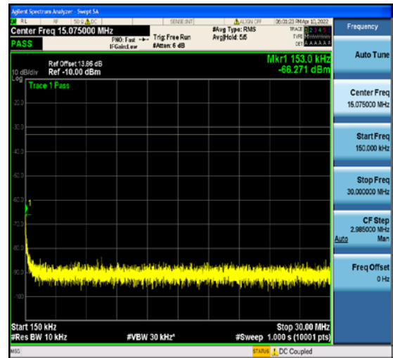
1-N2-PC3-15-10-H-5-DFT-QPSK-Edge_1RB _Right-1@51-0.15-30-Ant1--66.27--33-PASS
