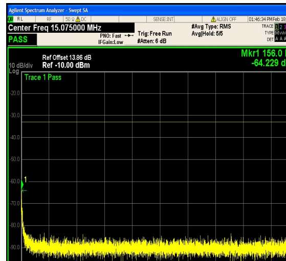
1-N25-PC3-15-5-L-8-DFT-16QAM-Edge_1R B_Right-1@24-0.15-30-Ant1--64.23--33-PAS S
