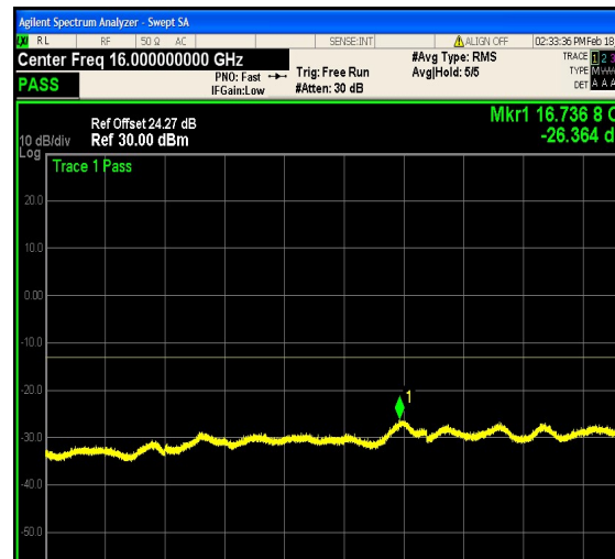
1-N25-PC3-15-5-M-14-DFT-256QAM-Edge_ 1RB_Right-1@24-12000-20000-Ant1--26.36- -13-PASS
