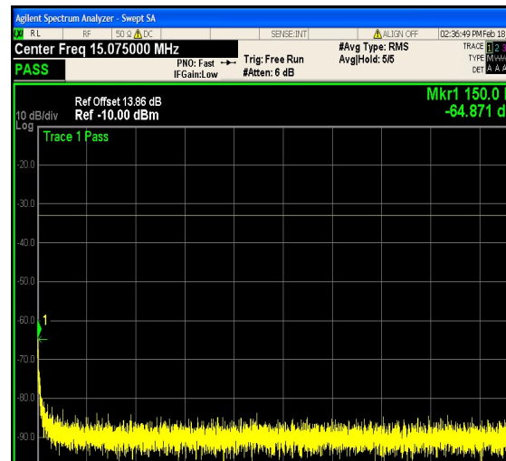
1-N25-PC3-15-5-M-17-CP-QPSK-Edge_1RB _Right-1@24-0.15-30-Ant1--64.87--33-PASS
