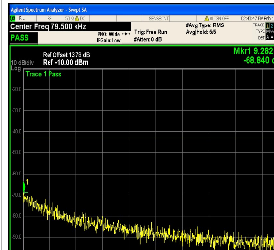
1-N25-PC3-15-5-M-20-CP-16QAM-Edge_1R B_Right-1@24-0.009-0.15-Ant1--68.84--43-P ASS
