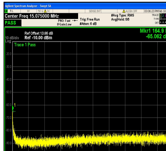
1-N25-PC3-15-5-H-11-DFT-64QAM-Edge_1R B_Right-1@24-0.15-30-Ant1--65.06--33-PAS S
