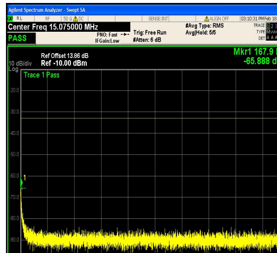
1-N25-PC3-15-5-H-14-DFT-256QAM-Edge_1 RB_Right-1@24-0.15-30-Ant1--65.89--33-PA SS
