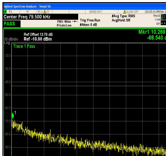
1-N25-PC3-15-5-H-25-CP-256QAM-Edge_1 RB_Left-1@0-0.009-0.15-Ant1--68.54--43-PA SS
