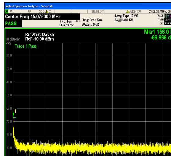
1-N25-PC3-15-10-M-21-CP-16QAM-Outer_F ull-52@0-0.15-30-Ant1--66.97--33-PASS
