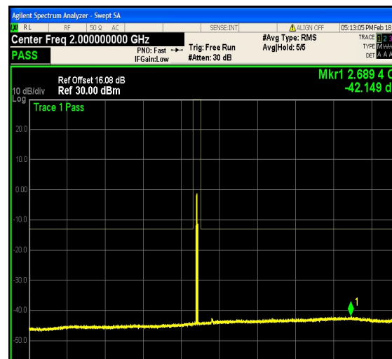
1-N25-PC3-15-10-M-24-CP-64QAM-Outer_F ull-52@0-0.15-30-Ant1--65.94--33-PASS
