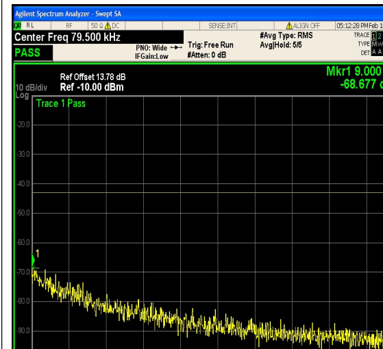
1-N25-PC3-15-10-M-24-CP-64QAM-Outer_F ull-52@0-0.009-0.15-Ant1--68.68--43-PASS
