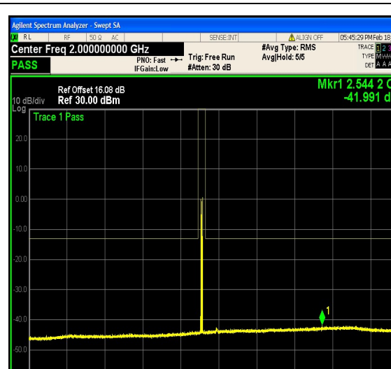
1-N25-PC3-15-10-H-20-CP-16QAM-Edge_1 RB_Right-1@51-1000-3000-Ant1--41.99--13- PASS
