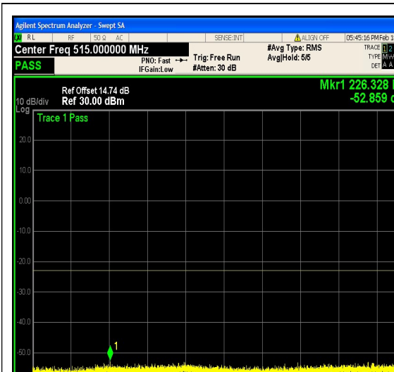
1-N25-PC3-15-10-H-20-CP-16QAM-Edge_1 RB_Right-1@51-30-1000-Ant1--52.86--23-P ASS
