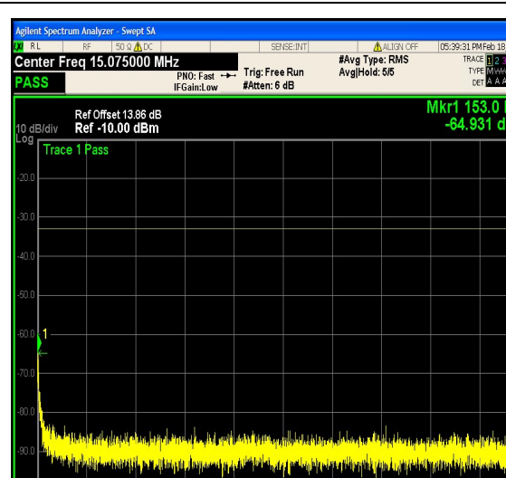
1-N25-PC3-15-10-H-16-CP-QPSK-Edge_1R B_Left-1@0-0.15-30-Ant1--64.93--33-PASS
