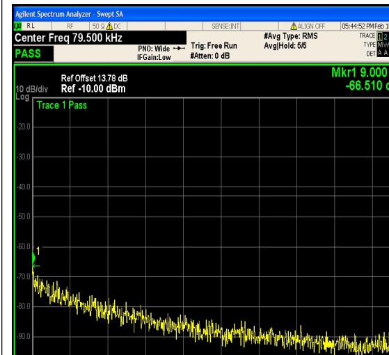
1-N25-PC3-15-10-H-20-CP-16QAM-Edge_1 RB_Right-1@51-0.009-0.15-Ant1--66.51--43- PASS
