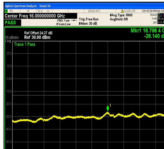
1-N25-PC3-15-10-H-20-CP-16QAM-Edge_1 RB_Right-1@51-12000-20000-Ant1--26.14-- 13-PASS
