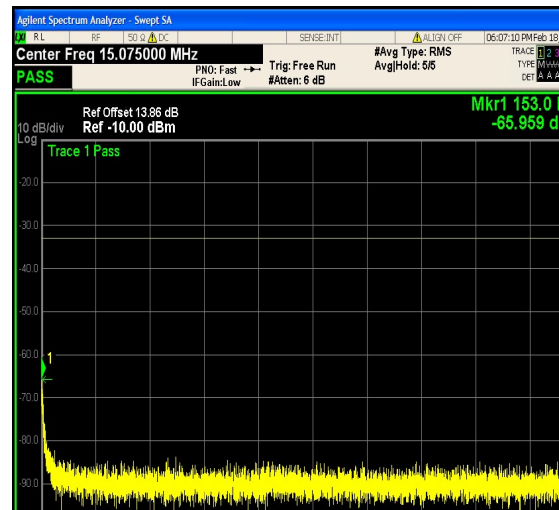
1-N25-PC3-15-15-L-5-DFT-QPSK-Edge_1RB _Right-1@78-0.15-30-Ant1--65.96--33-PASS
