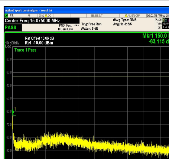
1-N25-PC3-15-15-L-3-DFT-PI2BPSK-Out_ Full-75@0-0.15-30-Ant1--63.12--33-PASS
