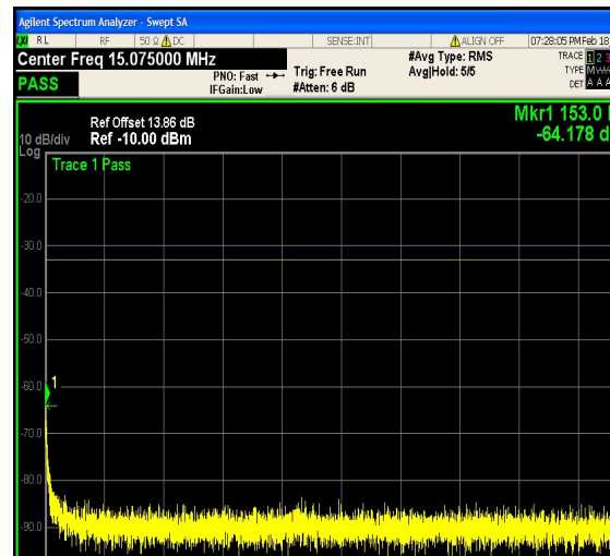
1-N25-PC3-15-15-M-16-CP-QPSK-Edge_1R B_Left-1@0-0.15-30-Ant1--64.18--33-PASS
