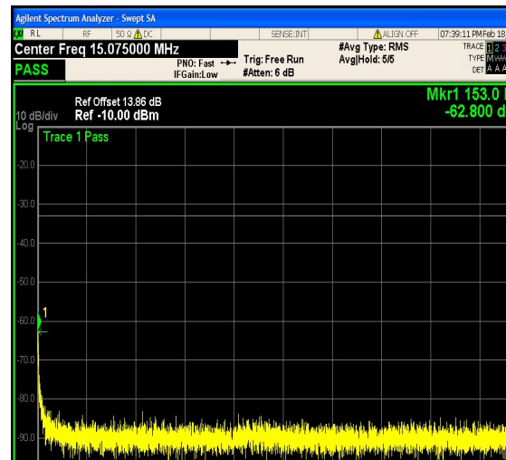
1-N25-PC3-15-15-M-24-CP-64QAM-Outer_F ull-79@0-0.15-30-Ant1--62.80--33-PASS
