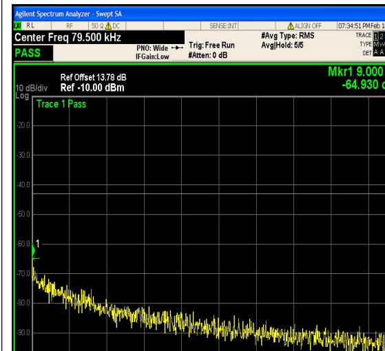
1-N25-PC3-15-15-M-21-CP-16QAM-Outer_F ull-79@0-0.009-0.15-Ant1--64.93--43-PASS
