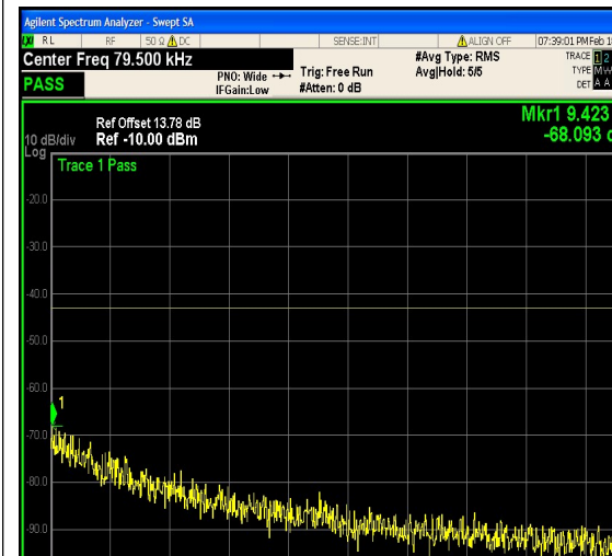
1-N25-PC3-15-15-M-24-CP-64QAM-Outer_F ull-79@0-0.009-0.15-Ant1--68.09--43-PASS
