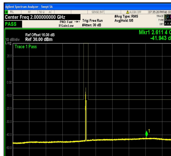
1-N25-PC3-15-15-M-21-CP-16QAM-Outer_F ull-79@0-0.15-30-Ant1--64.88--33-PASS
