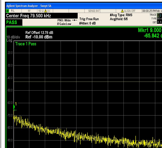
1-N25-PC3-15-15-H-12-DFT-64QAM-Outer_ Full-75@0-0.009-0.15-Ant1--65.84--43-PASS
