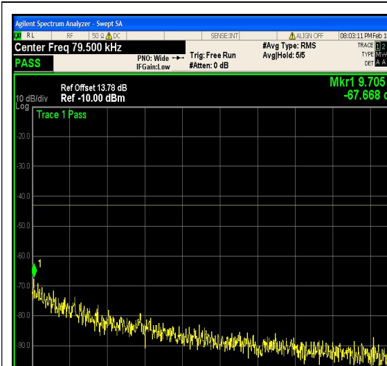
1-N25-PC3-15-15-H-14-DFT-256QAM-Edge_ 1RB_Right-1@78-0.009-0.15-Ant1--67.67--4 3-PASS
