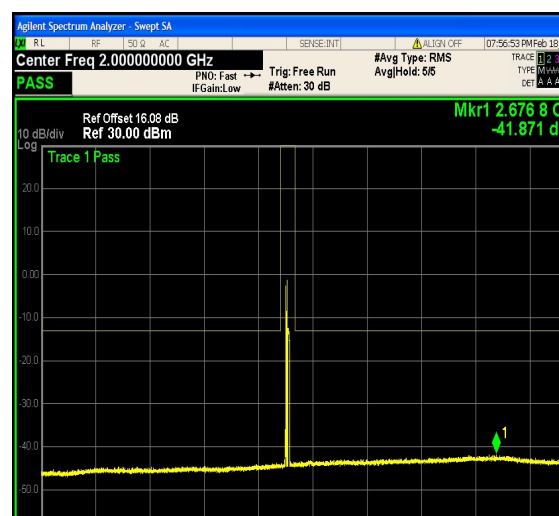
1-N25-PC3-15-15-H-9-DFT-16QAM-Outer_F ull-75@0-0.15-30-Ant1--63.38--33-PASS
