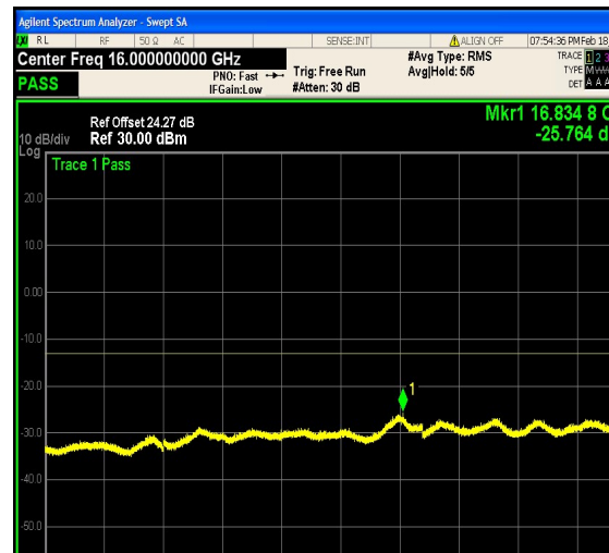
1-N25-PC3-15-15-H-7-DFT-16QAM-Edge_1 RB_Left-1@0-12000-20000-Ant1--25.76--13- PASS
