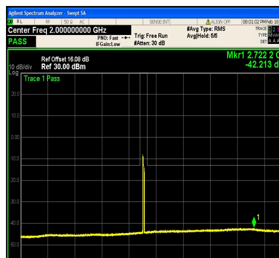
1-N25-PC3-15-15-H-12-DFT-64QAM-Outer_ Full-75@0-0.15-30-Ant1--64.01--33-PASS
