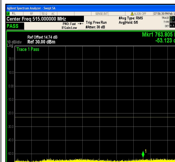
1-N25-PC3-15-15-H-9-DFT-16QAM-Outer_F ull-75@0-0.009-0.15-Ant1--69.46--43-PASS
