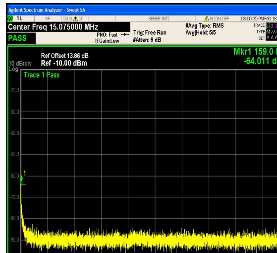
1-N25-PC3-15-15-H-12-DFT-64QAM-Outer_ Full-75@0-0.15-30-Ant1--64.01--33-PASS
