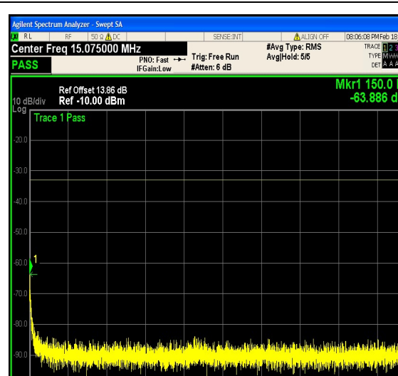
1-N25-PC3-15-15-H-16-CP-QPSK-Edge_1R B_Left-1@0-0.15-30-Ant1--63.89--33-PASS
