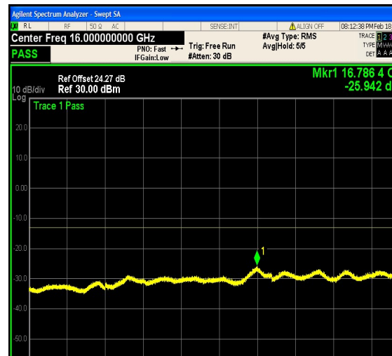
1-N25-PC3-15-15-H-20-CP-16QAM-Edge_1 RB_Right-1@78-12000-20000-Ant1--25.94-- 13-PASS
