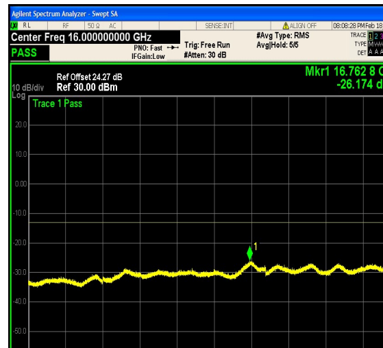
1-N25-PC3-15-15-H-17-CP-QPSK-Edge_1R B_Right-1@78-12000-20000-Ant1--26.17--13 -PASS
