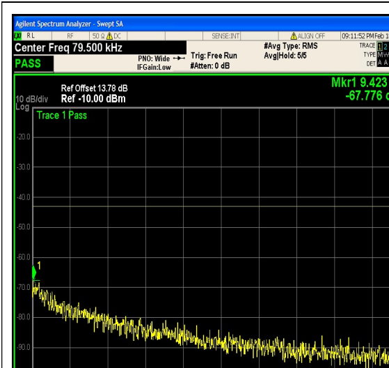
1-N25-PC3-15-20-L-26-CP-256QAM-Edge_1 RB_Right-1@105-0.009-0.15-Ant1--67.78--4 3-PASS
