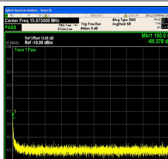
1-N25-PC3-15-20-L-26-CP-256QAM-Edge_1 RB_Right-1@105-0.15-30-Ant1--65.38--33-P ASS
