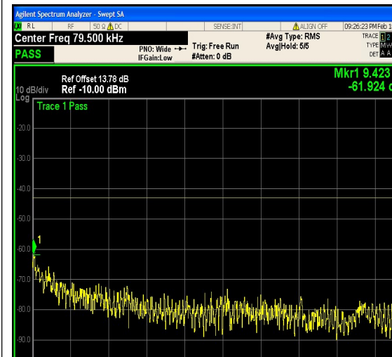
1-N25-PC3-15-20-M-9-DFT-16QAM-Outer_F ull-100@0-0.009-0.15-Ant1--61.92--43-PASS
