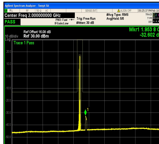
1-N25-PC3-15-20-M-8-DFT-16QAM-Edge_1 RB_Right-1@105-1000-3000-Ant1--32.60--1 3-PASS
