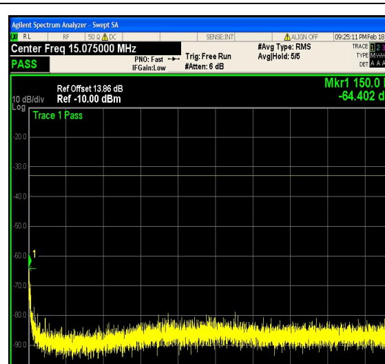
1-N25-PC3-15-20-M-8-DFT-16QAM-Edge_1 RB_Right-1@105-0.15-30-Ant1--64.40--33-P ASS
