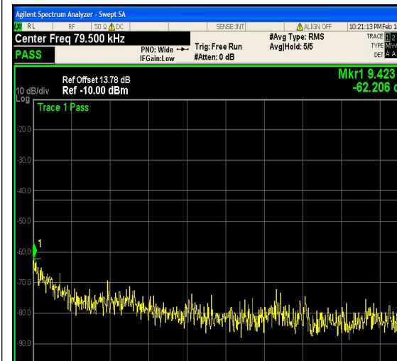
1-N25-PC3-15-20-H-21-CP-16QAM-Outer_F ull-106@0-0.009-0.15-Ant1--62.21--43-PASS
