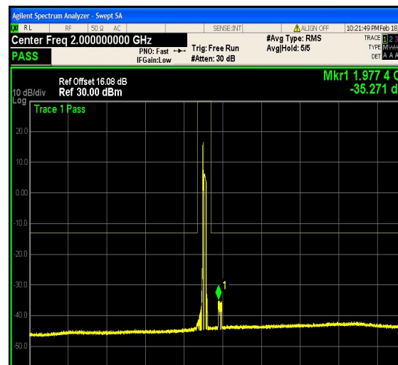
1-N25-PC3-15-20-H-21-CP-16QAM-Outer_F ull-106@0-0.15-30-Ant1--66.00--33-PASS
