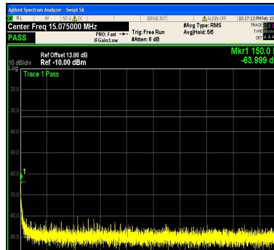
1-N25-PC3-15-20-H-18-CP-QPSK-Outer_Ful I-106@0-0.15-30-Ant1--64.00--33-PASS
