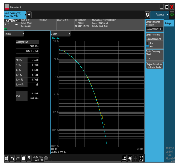
1-N41-PC2-30-40-M-6-CP-QPSK-Out_ Full-100@0-8.45-100%-0.00-8.45-PASS-≤13
