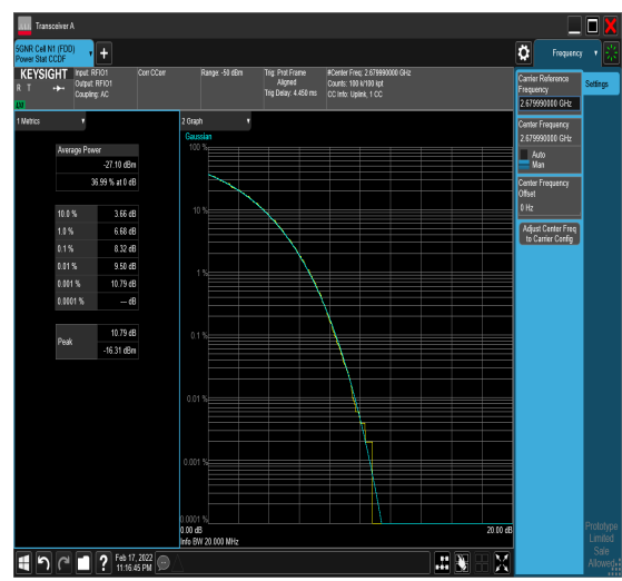
1-N41-PC2-30-20-H-6-CP-QPSK-Out_Full- 51@0-8.32-100%-0.00-8.32-PASS-≤13
