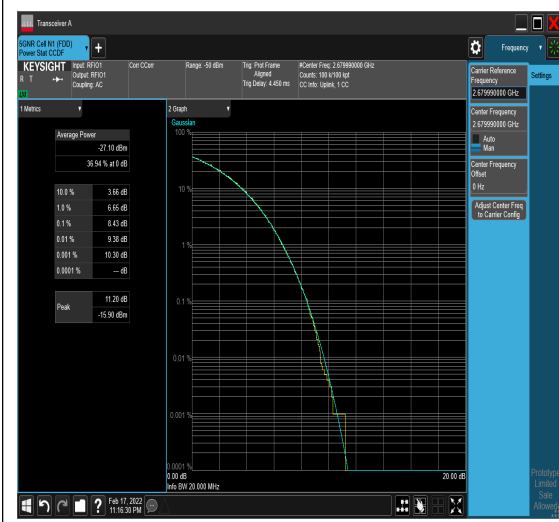
1-N41-PC2-30-20-H-5-DFT-256QAM-Out_F ull-50@0-8.43-100%-0.00-8.43-PASS-≤13
