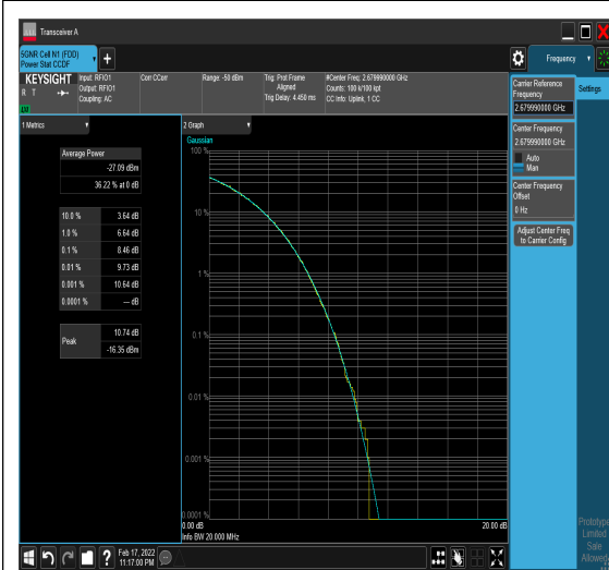
1-N41-PC2-30-20-H-7-CP-16QAM-Out_Ful
