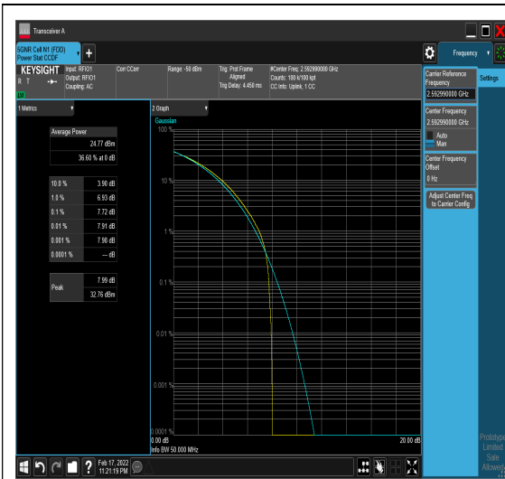
1-N41-PC2-30-40-M-1-DFT-PI2BPSK-Out_ Full-100@0-7.72-100%-0.00-7.72-PASS-≤13
