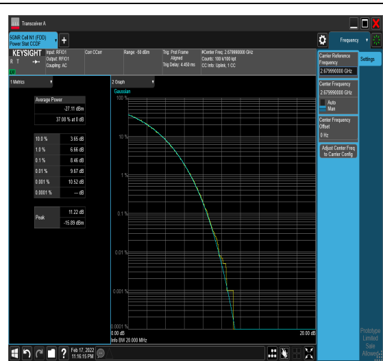
1-N41-PC2-30-20-H-4-DFT-64QAM-Out_F ull-50@0-8.46-100%-0.00-8.46-PASS-≤13
