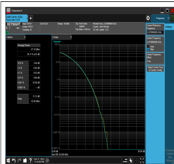
1-N41-PC2-30-20-H-3-DFT-16QAM-Out_F ull-50@0-8.52-100%-0.00-8.52-PASS-≤13
