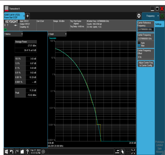
1-N41-PC2-30-20-H-8-CP-64QAM-Out_Ful
