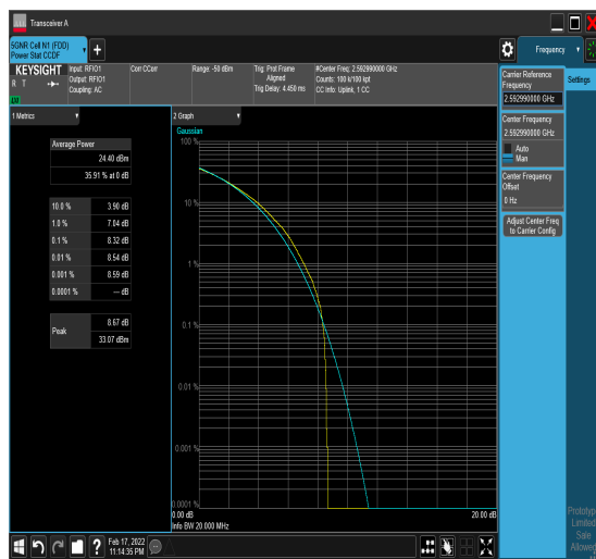
1-N41-PC2-30-20-M-8-CP-64QAM-Outer_Full-51@0-8.32-100%-0.00-8.32-PASS-≤13
