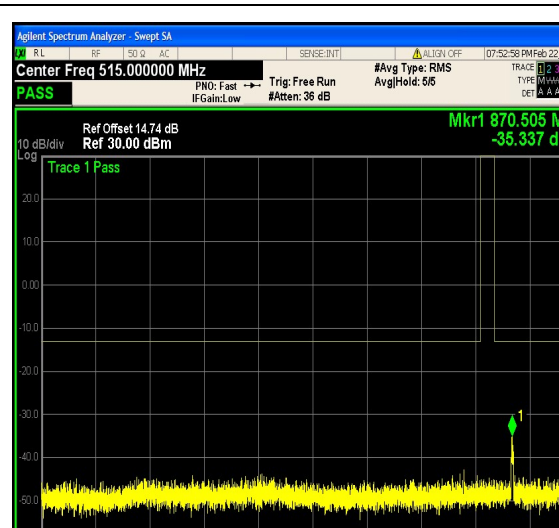
1-N5-PC3-15-5-L-18-CP-QPSK-Outet_Full-2 5@0-30-1000-Ant1--35.34--13-PASS
