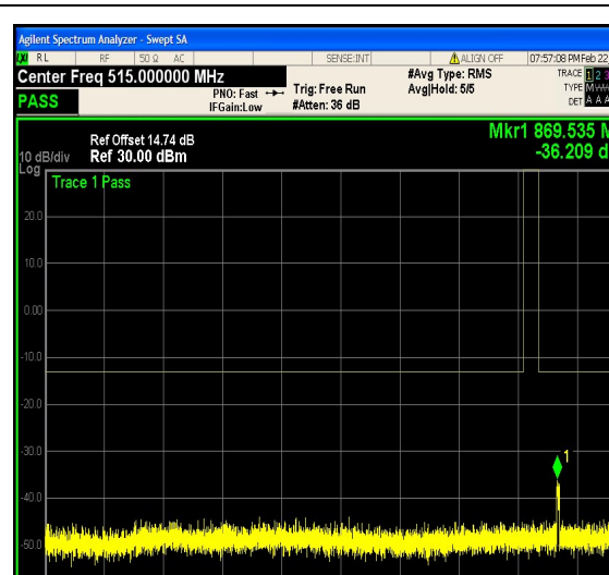
1-N5-PC3-15-5-L-20-CP-16QAM-Edge_1RB _Right-1@24-30-1000-Ant1--36.21--13-PASS
