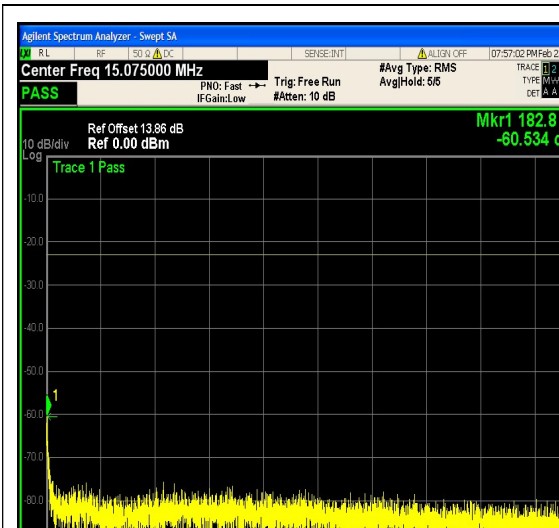
1-N5-PC3-15-5-L-20-CP-16QAM-Edge_1RB _Right-1@24-0.15-30-Ant1--60.53--23-PASS
