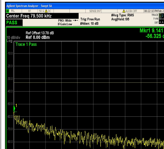
1-N5-PC3-15-5-M-12-DFT-64QAM-Outer_Ful l-25@0-0.009-0.15-Ant1--56.33--33-PASS
