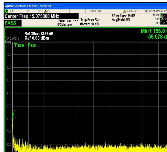
1-N5-PC3-15-5-M-12-DFT-64QAM-Outer_Ful l-25@0.15-30-Ant1--59.08--23-PASS
