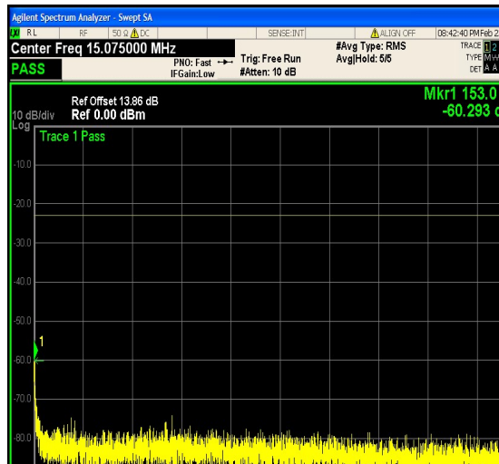
1-N5-PC3-15-5-H-4-DFT-QPSK-Edge_1RB_ Left-1@0-0.15-30-Ant1--60.29--23-PASS
