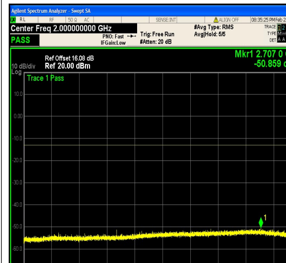
1-N5-PC3-15-5-M-27-CP-256QAM-Outer_Ful I-25@0-1000-3000-Ant1--50.86--13-PASS
