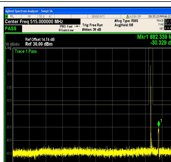
1-N5-PC3-15-5-M-27-CP-256QAM-Outer_Ful I-25@0-30-1000-Ant1--30.33--13-PASS
