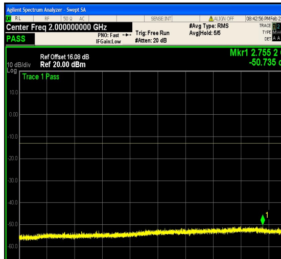
1-N5-PC3-15-5-H-4-DFT-QPSK-Edge_1RB_ Left-1@0-1000-3000-Ant1--50.73--13-PASS
