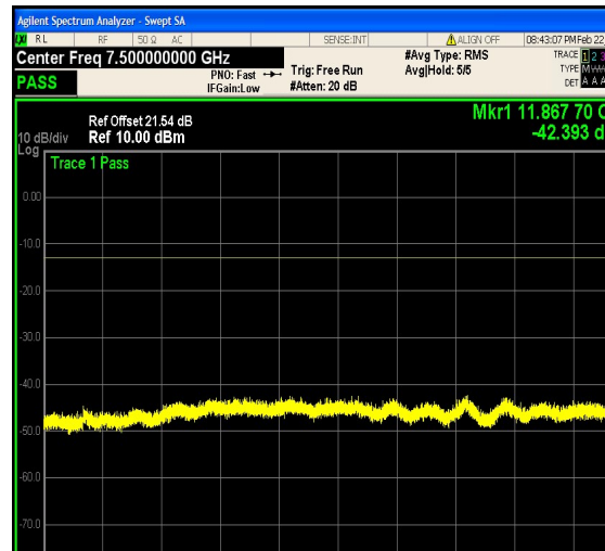
1-N5-PC3-15-5-H-4-DFT-QPSK-Edge_1RB_ Left-1@0-3000-12000-Ant1--42.39--13-PASS
