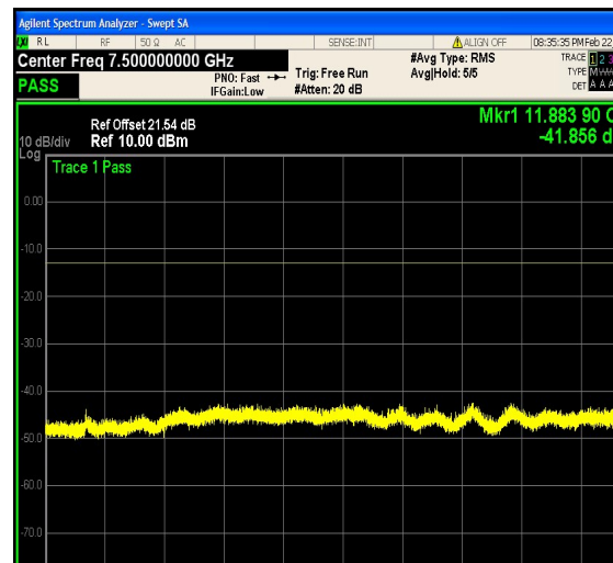
1-N5-PC3-15-5-M-27-CP-256QAM-Outer_Ful I-25@0-3000-12000-Ant1--41.86--13-PASS
