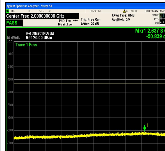
1-N5-PC3-15-5-H-14-DFT-256QAM-Edge_1 RB_Right-1@24-1000-3000-Ant1--50.84--13- PASS
