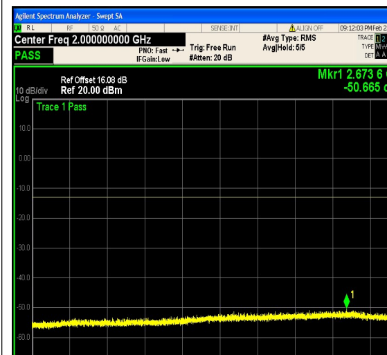
1-N5-PC3-15-5-H-18-CP-QPSK-Outer_Full-2 5@0-1000-3000-Ant1--50.66--13-PASS
