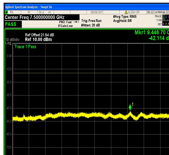
1-N5-PC3-15-5-H-18-CP-QPSK-Outer_Full-2 5@0-3000-12000-Ant1--42.11--13-PASS
