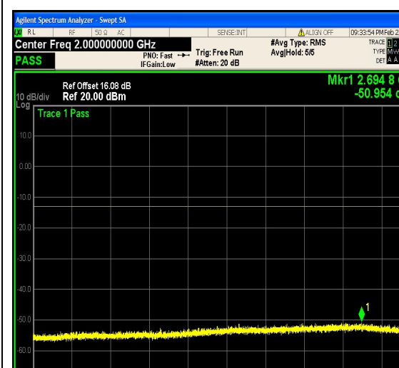
1-N5-PC3-15-10-L-3-DFT-PI2BPSK-Outer_F ull-50@0-0.15-30-Ant1--59.02--23-PASS
