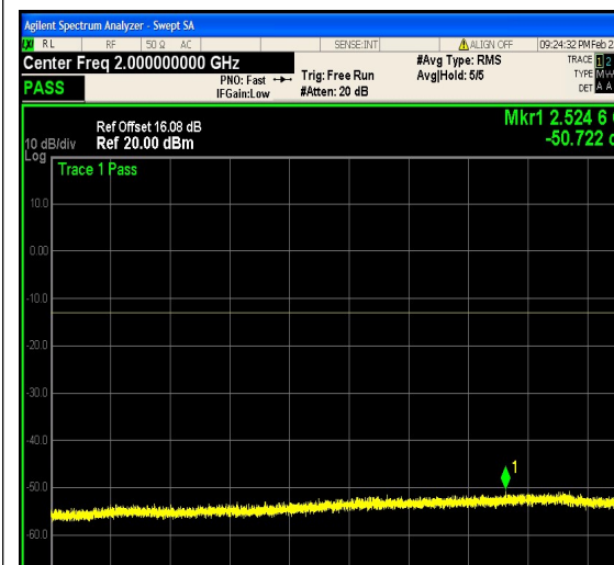
1-N5-PC3-15-5-H-24-CP-64QAM-Outer_Full- 25@0-1000-3000-Ant1--50.72--13-PASS
