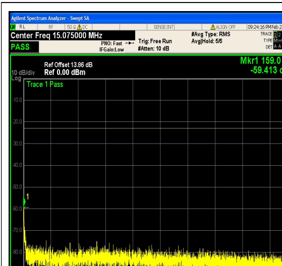
1-N5-PC3-15-5-H-24-CP-64QAM-Outer_Full- 25@0-0.15-30-Ant1--59.41--23-PASS
