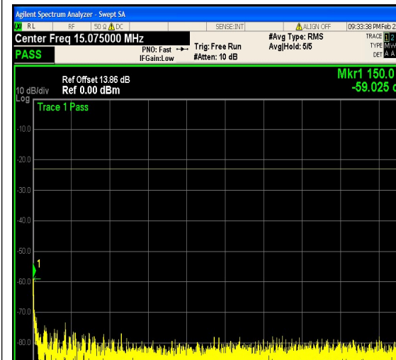
1-N5-PC3-15-10-L-3-DFT-PI2BPSK-Outer_F ull-50@0-0.15-30-Ant1--59.02--23-PASS
