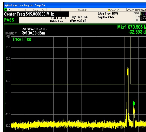
1-N5-PC3-15-10-L-3-DFT-PI2BPSK-Outer_F ull-50@0-30-1000-Ant1--32.89--13-PASS
