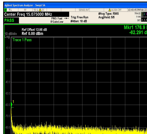
1-N5-PC3-15-10-M-27-CP-256QAM-Outer_F ull-52@0-0.15-30-Ant1--62.29--23-PASS
