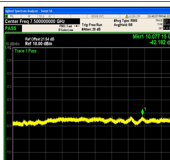
1-N5-PC3-15-10-M-26-CP-256QAM-Edge_1 RB_Right-1@51-3000-12000-Ant1--42.18--1 3-PASS
