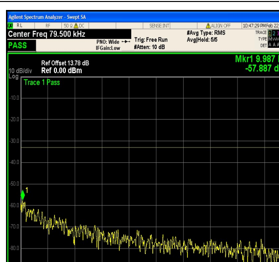
1-N5-PC3-15-10-M-26-CP-256QAM-Edge_1 RB_Right-1@51-0.009-0.15-Ant1--57.89--33- PASS
