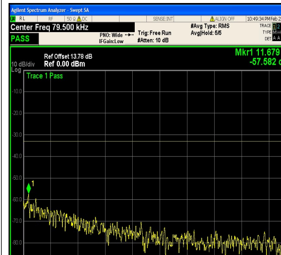
1-N5-PC3-15-10-M-27-CP-256QAM-Outer_F ull-52@0-0.009-0.15-Ant1--57.58--33-PASS
