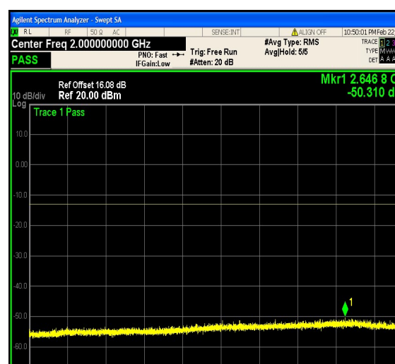
1-N5-PC3-15-10-M-27-CP-256QAM-Outer_F ull-52@0-0.15-30-Ant1--62.29--23-PASS
