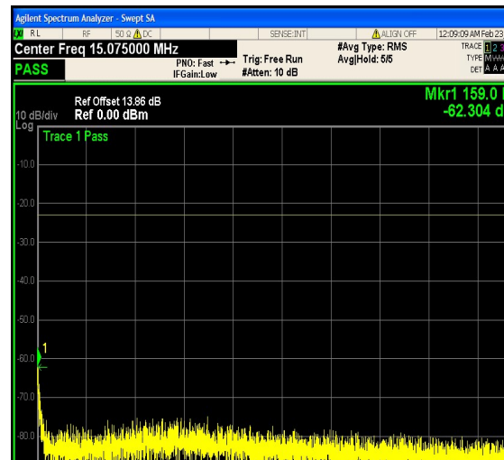
1-N5-PC3-15-15-L-27-CP-256QAM-Outer_F ull-79@0-0.15-30-Ant1--62.30--23-PASS
