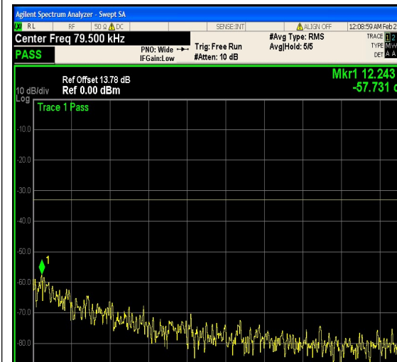
1-N5-PC3-15-15-L-27-CP-256QAM-Outer_F ull-79@0-0.009-0.15-Ant1--57.73--33-PASS
