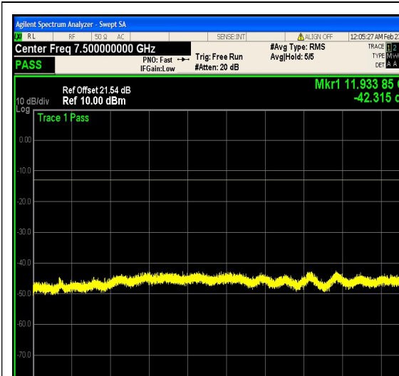
1-N5-PC3-15-15-L-25-CP-256QAM-Edge_1R B_Left-1@0-3000-12000-Ant1--42.31--13-PA SS
