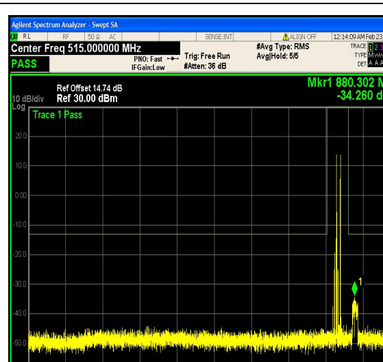
1-N5-PC3-15-15-M-5-DFT-QPSK-Edge_1RB _Right-1@78-30-1000-Ant1--34.26--13-PASS
