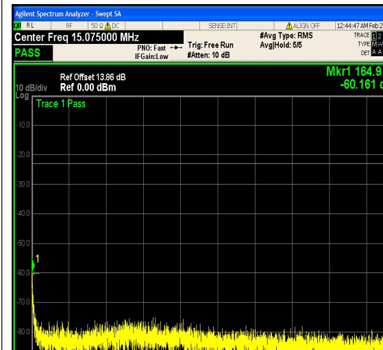
1-N5-PC3-15-15-H-6-DFT-QPSK-Outer_Full- 75@0-0.15-30-Ant1--60.16--23-PASS
