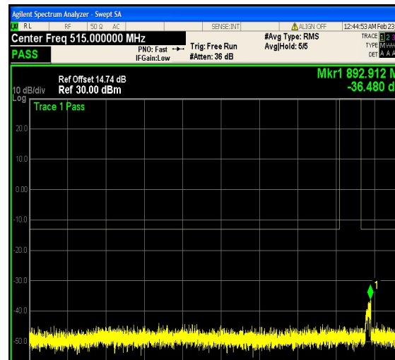
1-N5-PC3-15-15-H-6-DFT-QPSK-Outer_Full- 75@0-30-1000-Ant1--36.48--13-PASS
