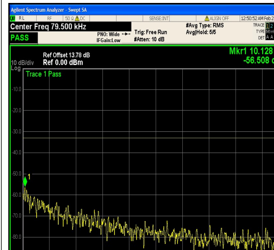
1-N5-PC3-15-15-H-9-DFT-16QAM-Outer_Ful l-75@0-0.009-0.15-Ant1--56.51--33-PASS
