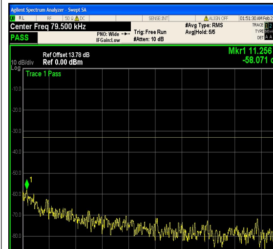
1-N5-PC3-15-20-L-26-CP-256QAM-Edge_1R B_Right-1@105-0.009-0.15-Ant1--58.07--33- PASS
