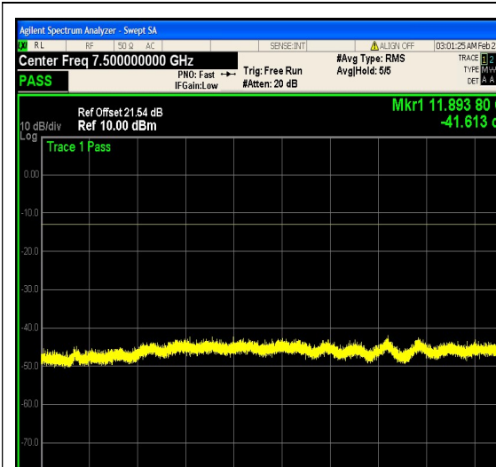
1-N5-PC3-15-20-H-14-DFT-256QAM-Edge_1 RB_Right-1@105-3000-12000-Ant1--41.61-- 13-PASS
