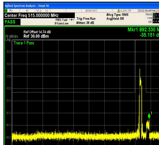
1-N5-PC3-15-20-H-15-DFT-256QAM-Outer_ Full-100@0-30-1000-Ant1--35.15--13-PASS
