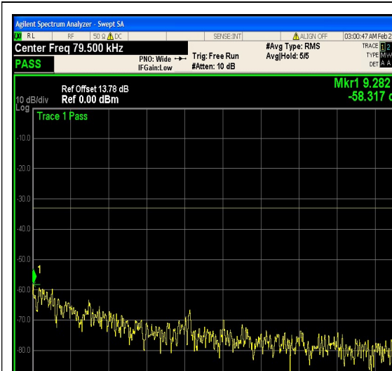
1-N5-PC3-15-20-H-14-DFT-256QAM-Edge_1 RB_Right-1@105-0.009-0.15-Ant1--58.32--3 3-PASS
