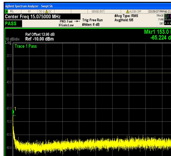
1-N66-PC3-15-5-L-14-DFT-256QAM-Edge_1 RB_Right-1@24-0.15-30-Ant1--65.22--33-PA SS
