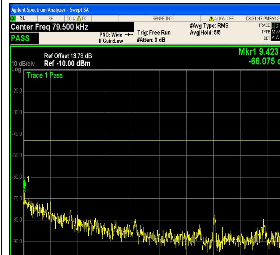
1-N66-PC3-15-5-M-2-DFT-PI2BPSK-Edge_1 RB_Right-1@24-0.009-0.15-Ant1--66.07--43- PASS
