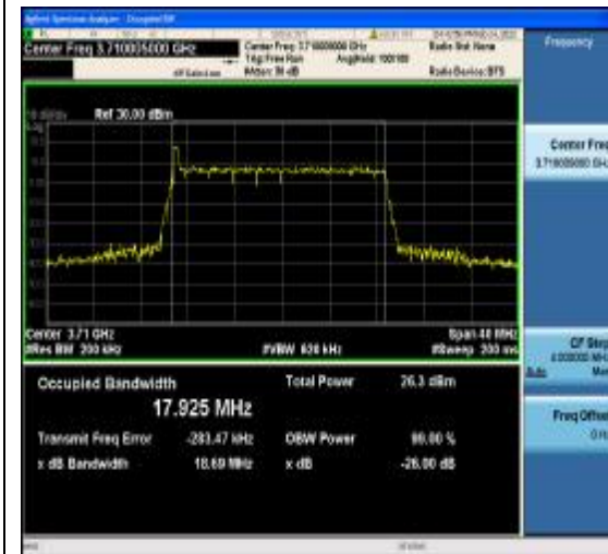
1-N77-3700-3980-PC2-30-20-L-7-CP-64QA M-Outer_Full-51@0-Ant1-17.925-18.69-≤20-PASS
