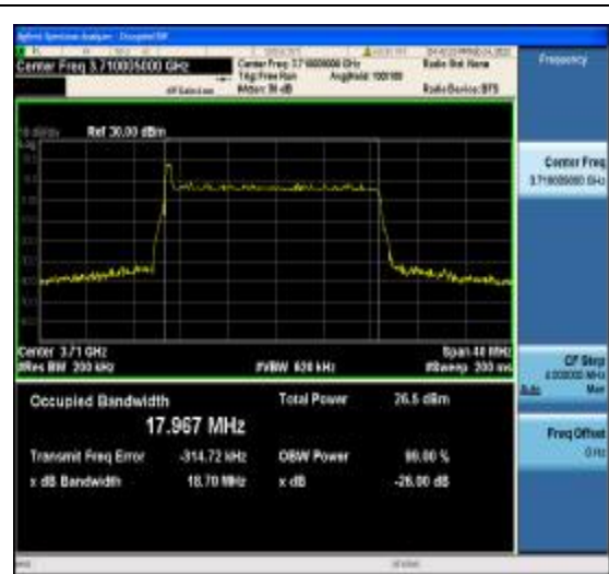
1-N77-3700-3980-PC2-30-20-L-6-CP-16QA M-Outer_Full-51@0-Ant1-17.967-18.70-≤20-PASS
