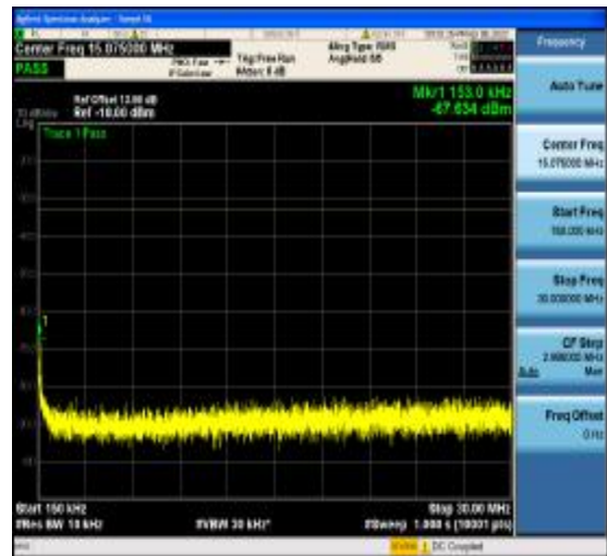
1-N77-3700-3980-PC2-30-20-M-8-DFT-16QA M-Edge_1RB_Right-1@50-0.15-30-Ant1--67.63--33-PASS
