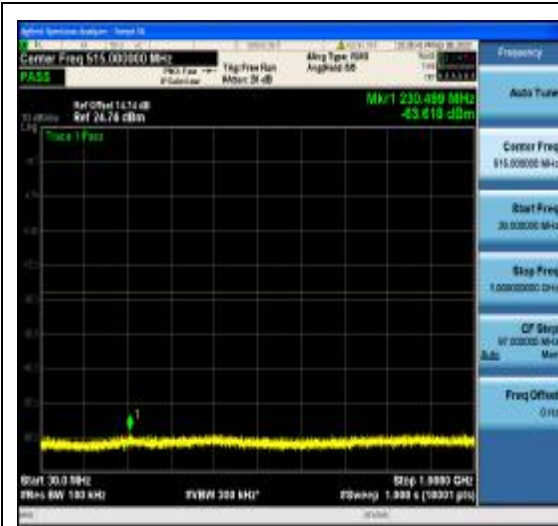
1-N77-3700-3980-PC2-30-20-H-25-CP-256Q AM-Edge_1RB_Left-1@0-30-1000-Ant1--63. 62--23-PASS
