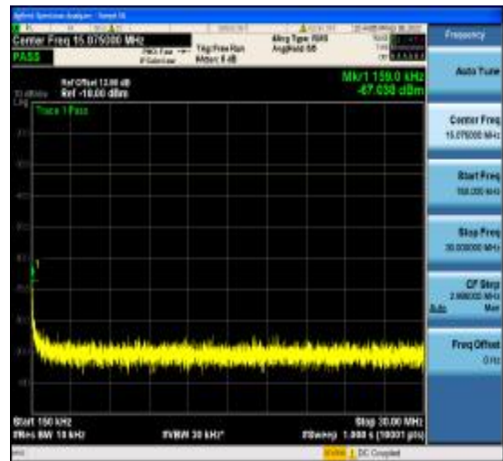
1-N77-3700-3980-PC2-30-40-L-6-DFT-QPSK -Outer_Full-100@0-0.15-30-Ant1--67.04--33- PASS
