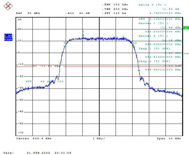
Band5-4183
