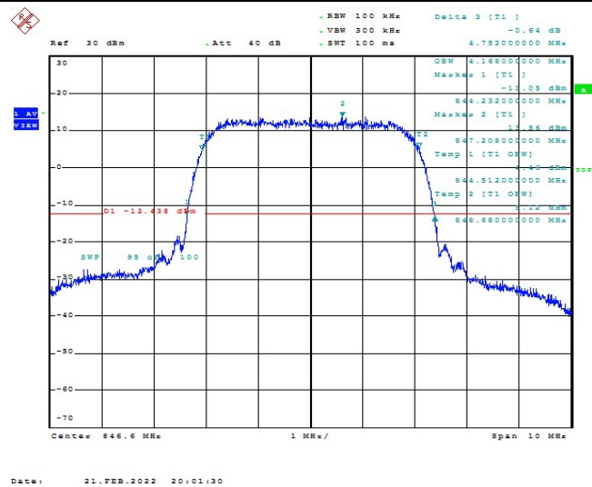
Band5-4233
