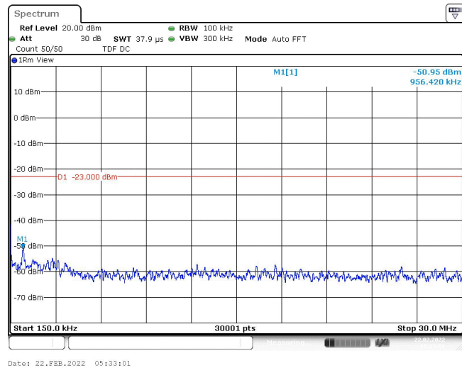
Band2-9400-2-0.15~30MHz
