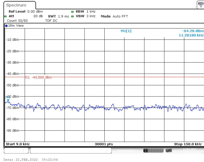
Band2-9400-2-0.009~0.15MHz
