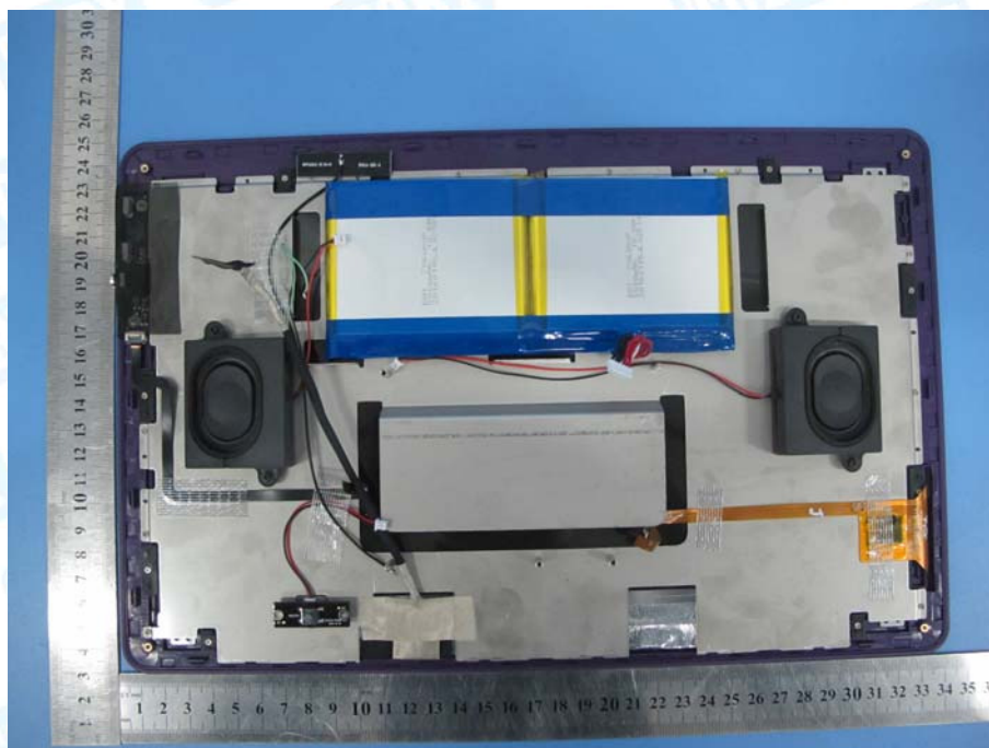
Photo 12 Appearance of Antenna
