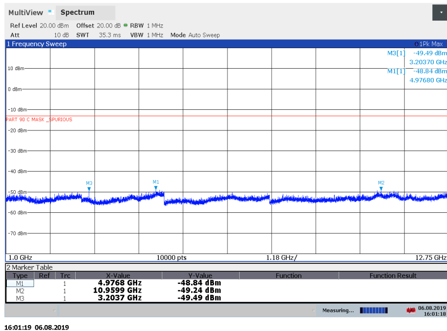
Plot 6: 1GHz to 12.75 GHz Highest channel
