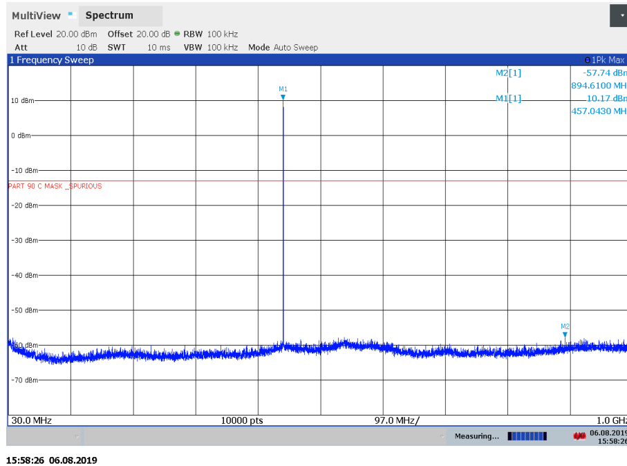
Plot 3: 30 MHz to 1 GHz Middle channel
