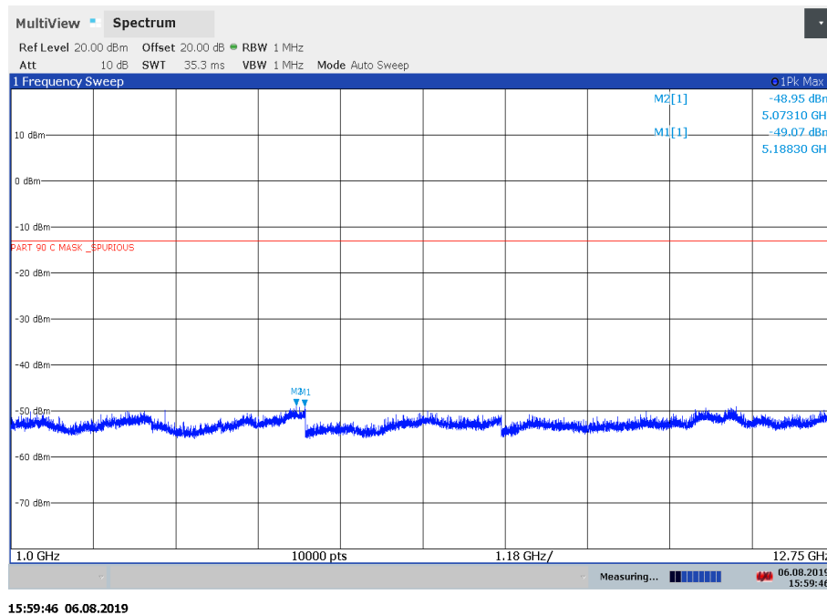
Plot 4: 1GHz to 12.75 GHz Middle channel
