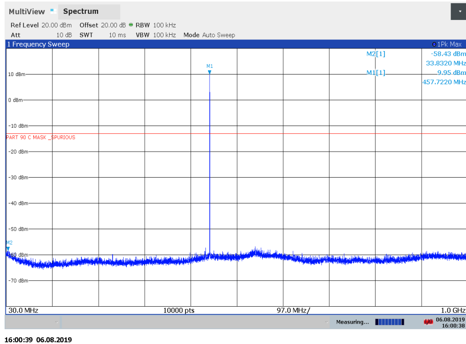
Plot 5: 30 MHz to 1 GHz Highest channel
