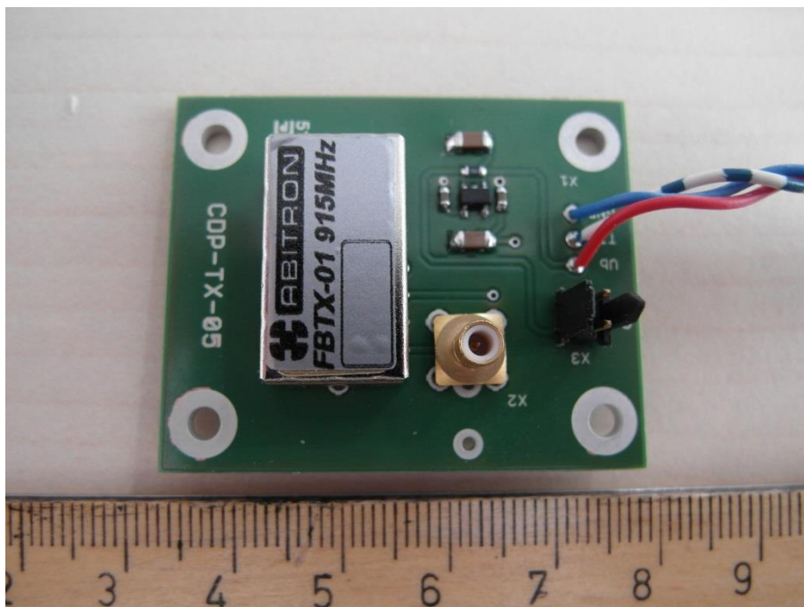
Photo 3: Front side of the EUT
