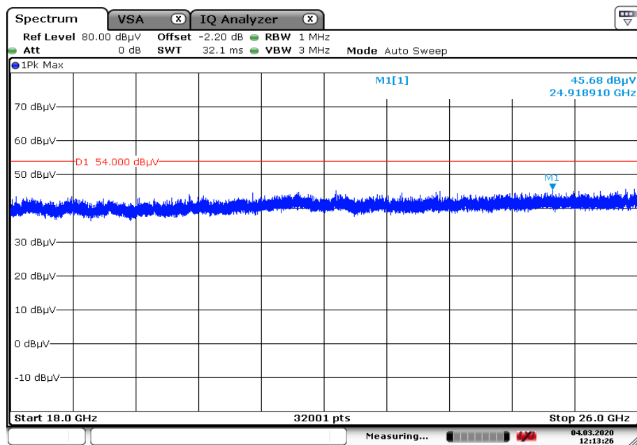
Plot 4: 18 GHz to 26 GHz, TX mode, 2440 MHz, vertical & horizontal polarization, 1 Msps S8 coded
