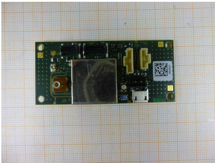
Photo 2: Module back side view
