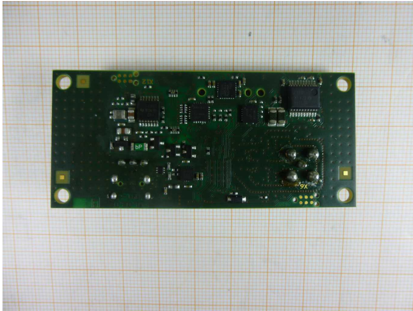
Photo 1: Module front side view
